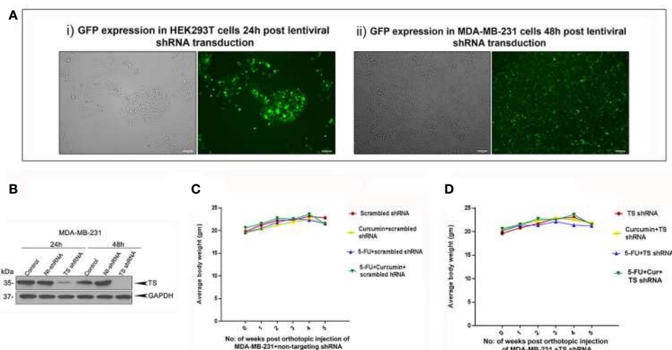
FIGURE 4 | Analysis of the efficiency of lentiviral transduction and expression status of TS in transduced cells. (A) Efficiency of lentiviral transduction in HEK 293T cells and successive infection in MDA-MB-231 cells, respectively as assessed by GFP expression. (B) Time-dependent analysis of expression status of TS in MDA-MB-231 cells transduced with TS shRNA compared to that of untreated control and cells transduced with control/non-targeting shRNA (Nt-shRNA) using immunoblotting. GAPDH levels are shown as the loading control. (C, D) Comparison of body weight from different treatment groups bearing MDA-MB-231 TS xenografts and MDA-MB-231 TS- xenografts, respectively.
